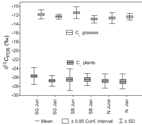
Fig. 1. Boxplot with means, 95 % confidence interval, and standard deviation (SD) of regional and seasonal carbon isotopic data for C 3 trees and forbs and C 4 grasses from Kruger National Park, collected during June 2002, January 2003, and June 2003. (SG = southern granites, SB = southern basalts; N = northern KNP).
