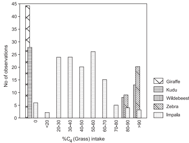
Fig. 2. Histogram combining specimens collected throughout Kruger National Park during June 2002, January 2003, and June 2003, showing reconstruction of %C 4 consumed, derived from herbivore faecal δ 13 C values using local vegetational data to define variance in isotopic end-points.
