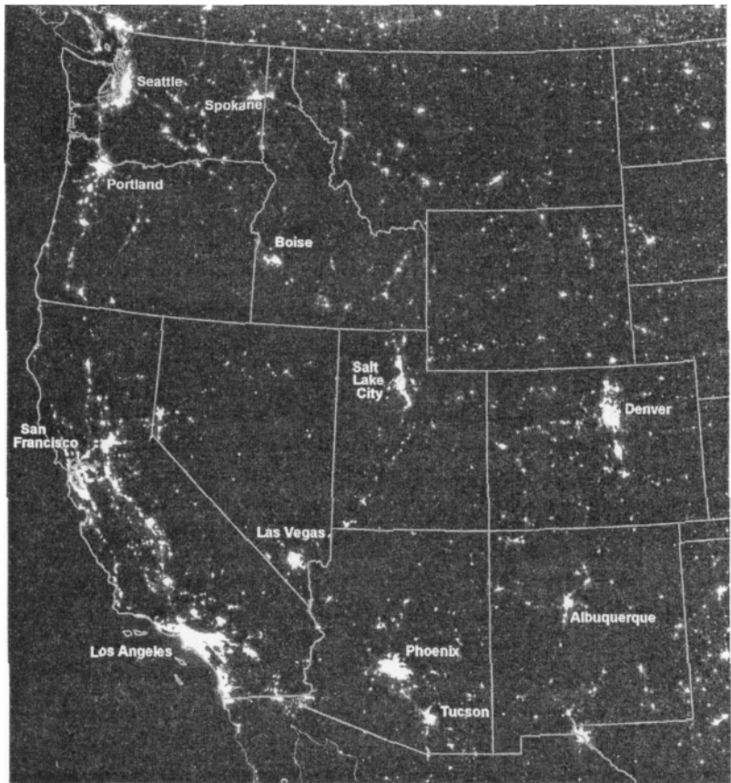
Figure 2.1 A nighttime satellite image of the West reveals a growing network of development against a dark background of open space.
