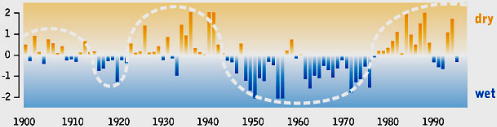
Pacific Decadal Oscillation, annual averages, 1900-1998
